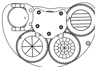
PRISM WHEEL 2
