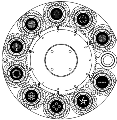
GOBO WHEEL 1
