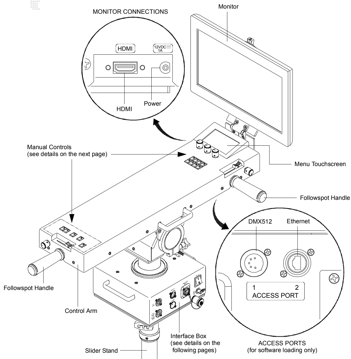
Figure 5: GC Followspot Controller - Main Components
