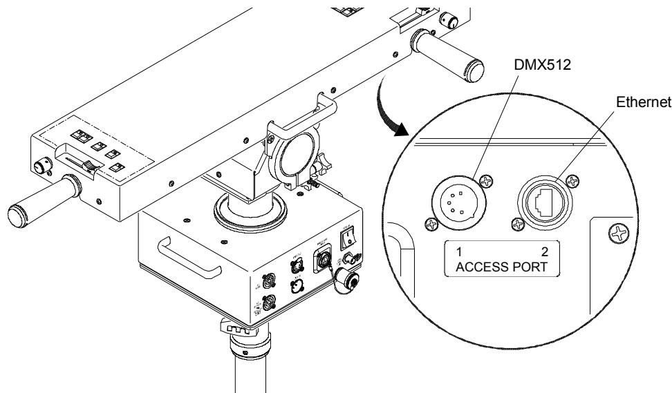
Figure 27: Access Ports
