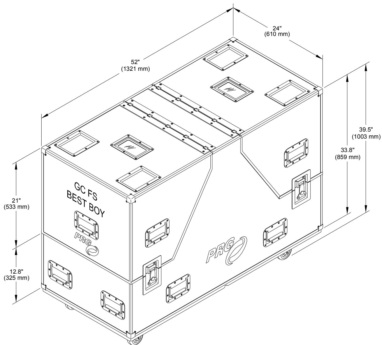
Figure 42: GC Best Boy Roadcase Dimensions
