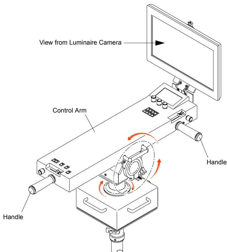
Figure 22: Pan/Tilt Control
