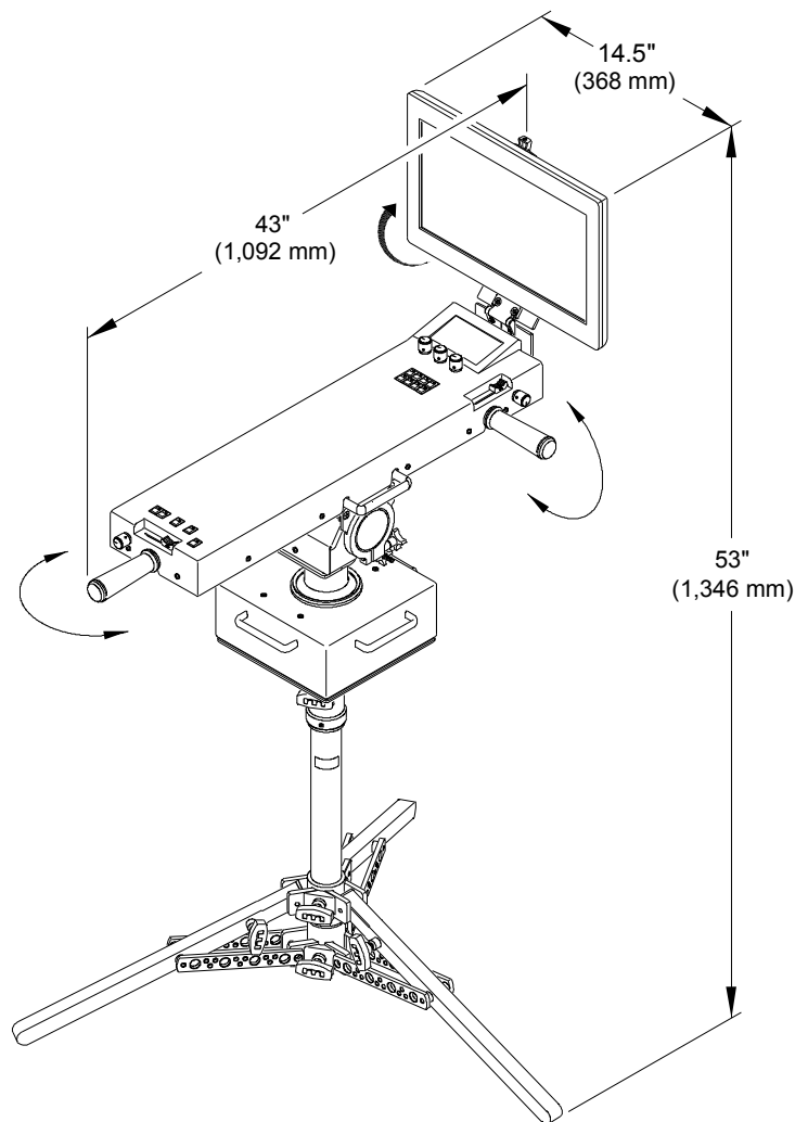
Figure 34: GC Followspot Controller Dimensions
