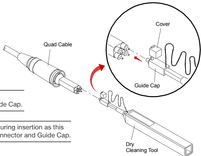
Figure 30: Quad Cable Connector Cleaning (Field)
