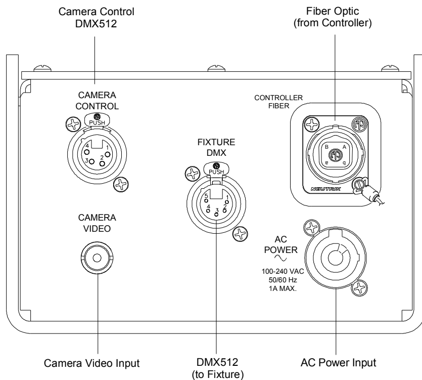
Figure 8: Truss Box Interface Panel
