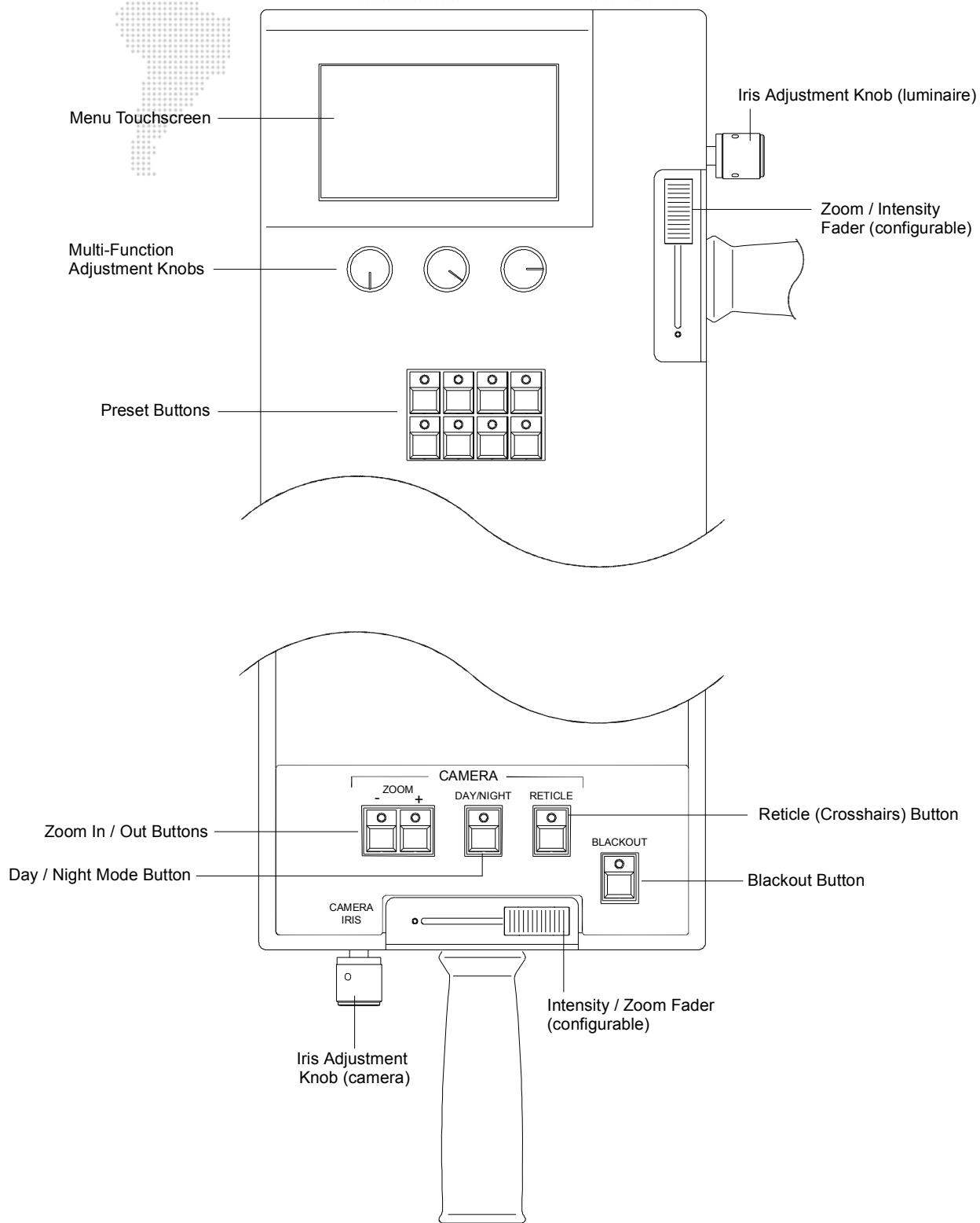
Figure 6: GC Followspot Controller - Control Arm Details
