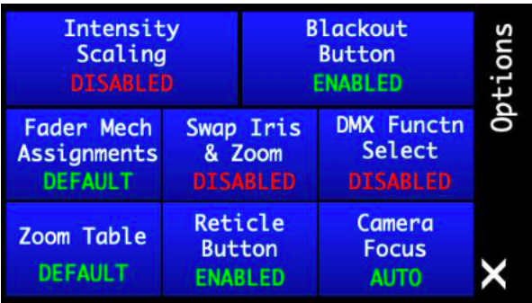
Figure A-1: Options Window With New Function Select Button
