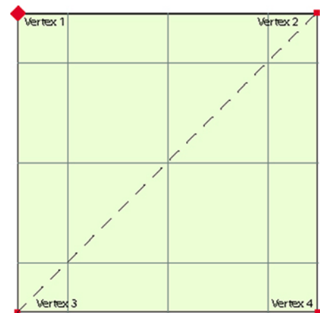
Equivalent Triangle Strip Screen Object
