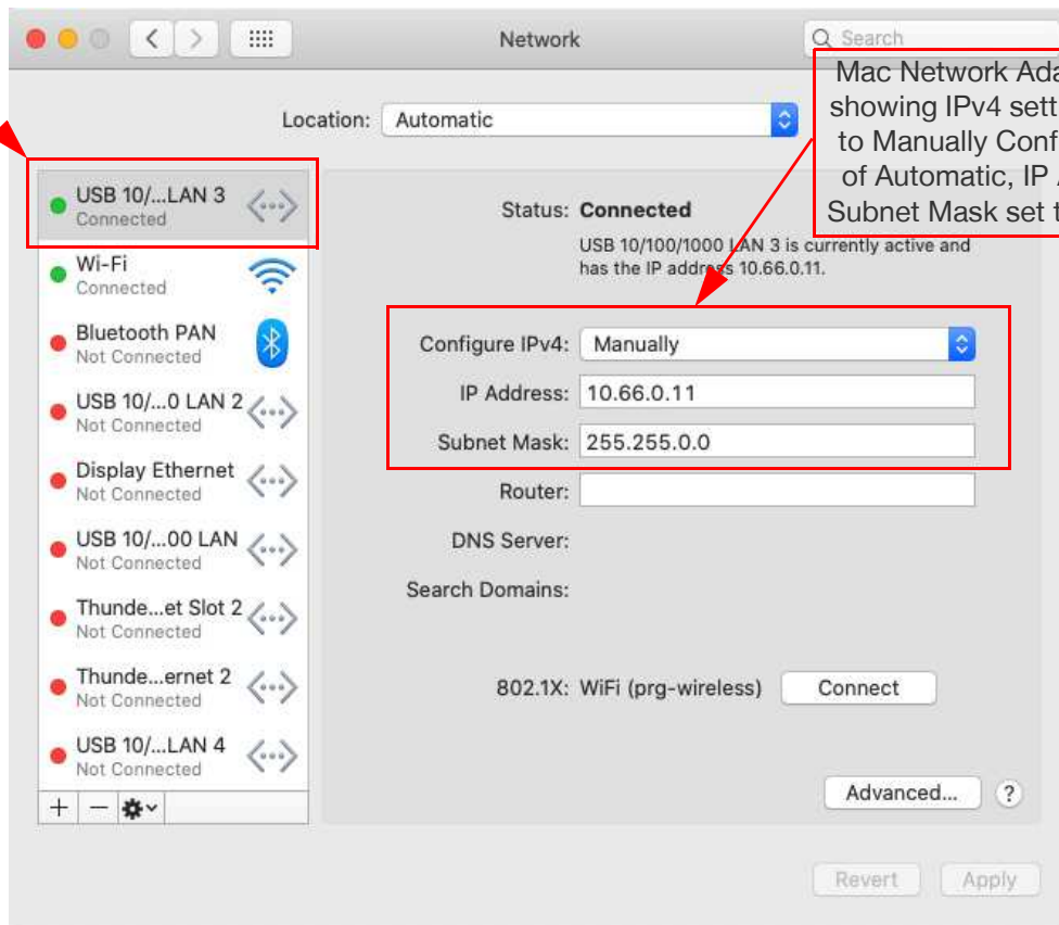
Figure 55: Configuring a Mac Network Adapter to Connect S400ToolsFX
